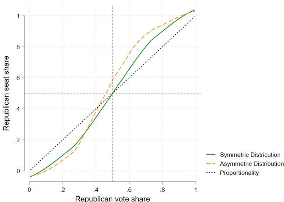
Figure 7: Hypothetical symmetric vote-seat curve
